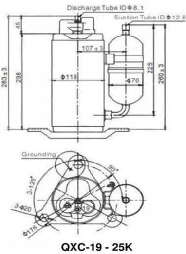
QXC-19 - 25K
